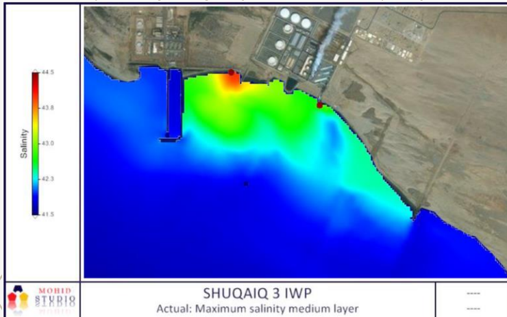
Shuqaiq 3 desalination plant (Saudi Arabia). I.D.= 2.200 mm. Dilution studies.
