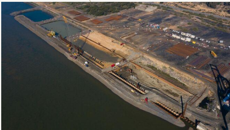
The northern expansion of the south quay, Huelva. (Spain)
