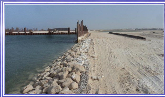
Extension of the Port of Nouadhibou, Mauritania (Sheetpiles)
